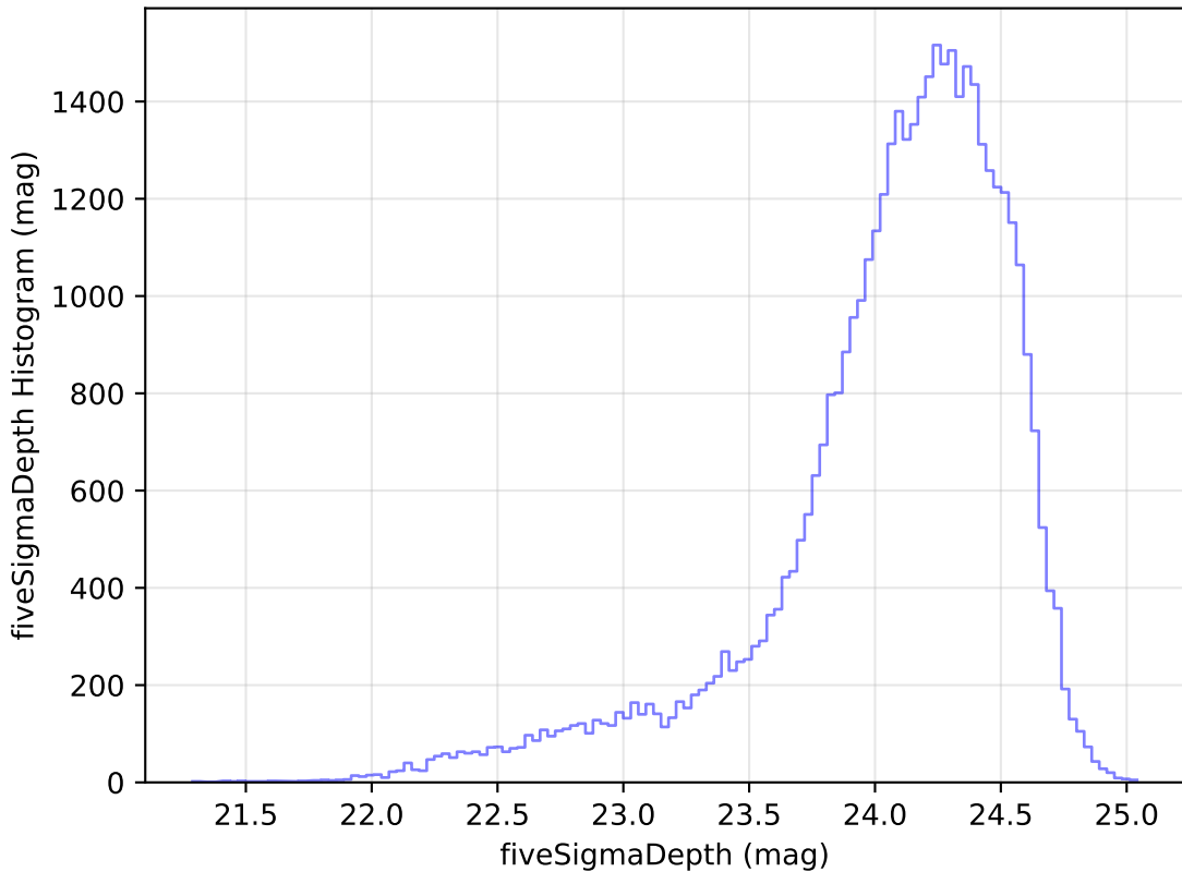
weather_cloudso20v3.4_10yrs Yr 1 r band: fiveSigmaDepth Histogram
