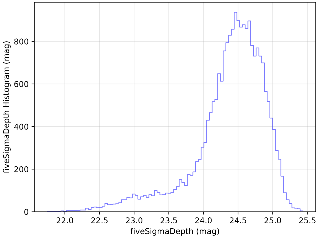
weather_cloudso20v3.4_10yrs Yr 1 g band: fiveSigmaDepth Histogram
