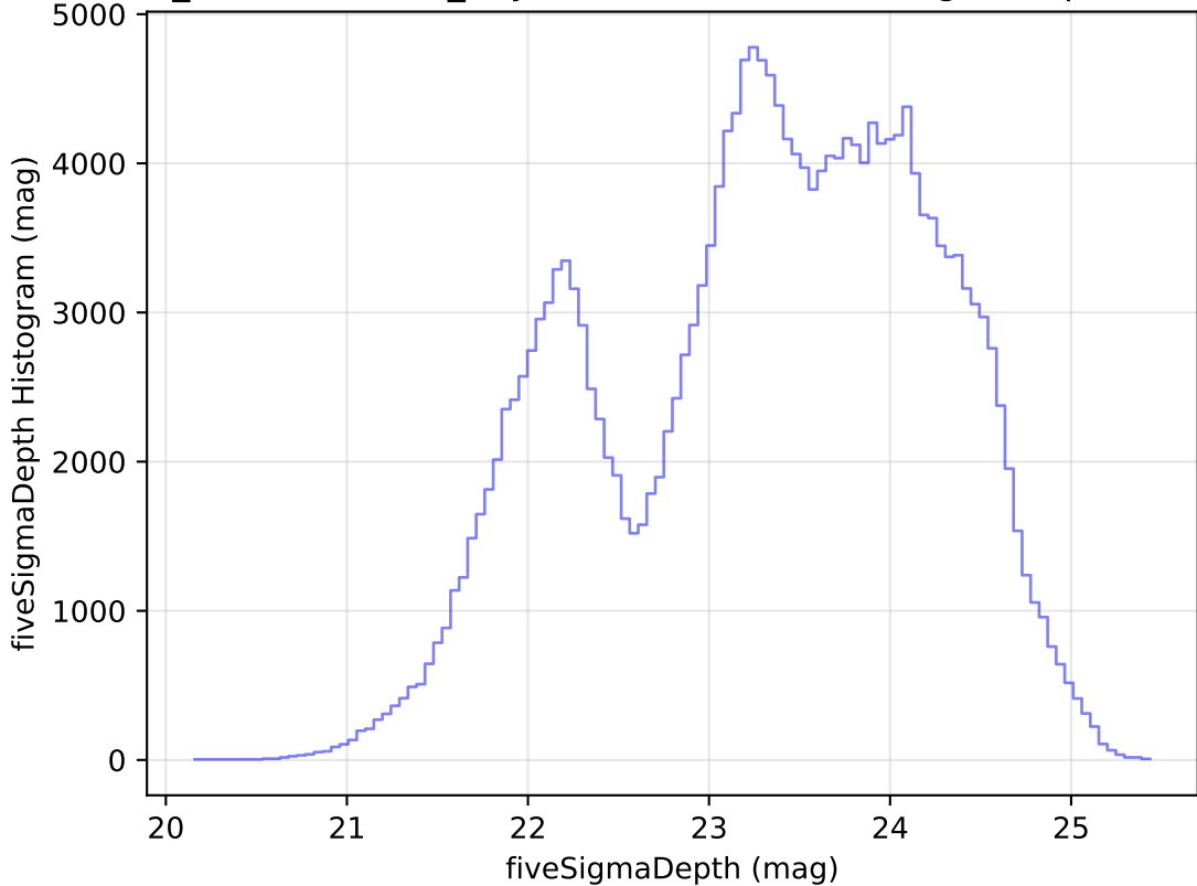
weather_cloudso20v3.4_10yrs Yr 1 all bands: fiveSigmaDepth Histogram
