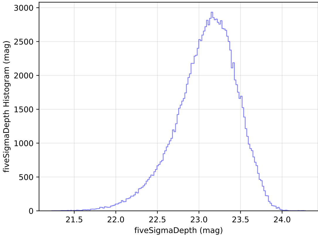
weather_cloudso20v3.4_10yrs WFD u band: fiveSigmaDepth Histogram
