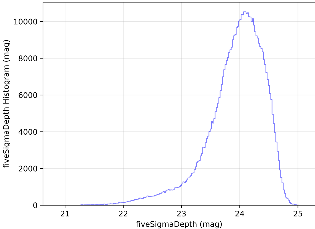
weather_cloudso20v3.4_10yrs WFD r band: fiveSigmaDepth Histogram
