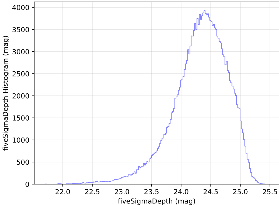
weather_cloudso20v3.4_10yrs WFD g band: fiveSigmaDepth Histogram
