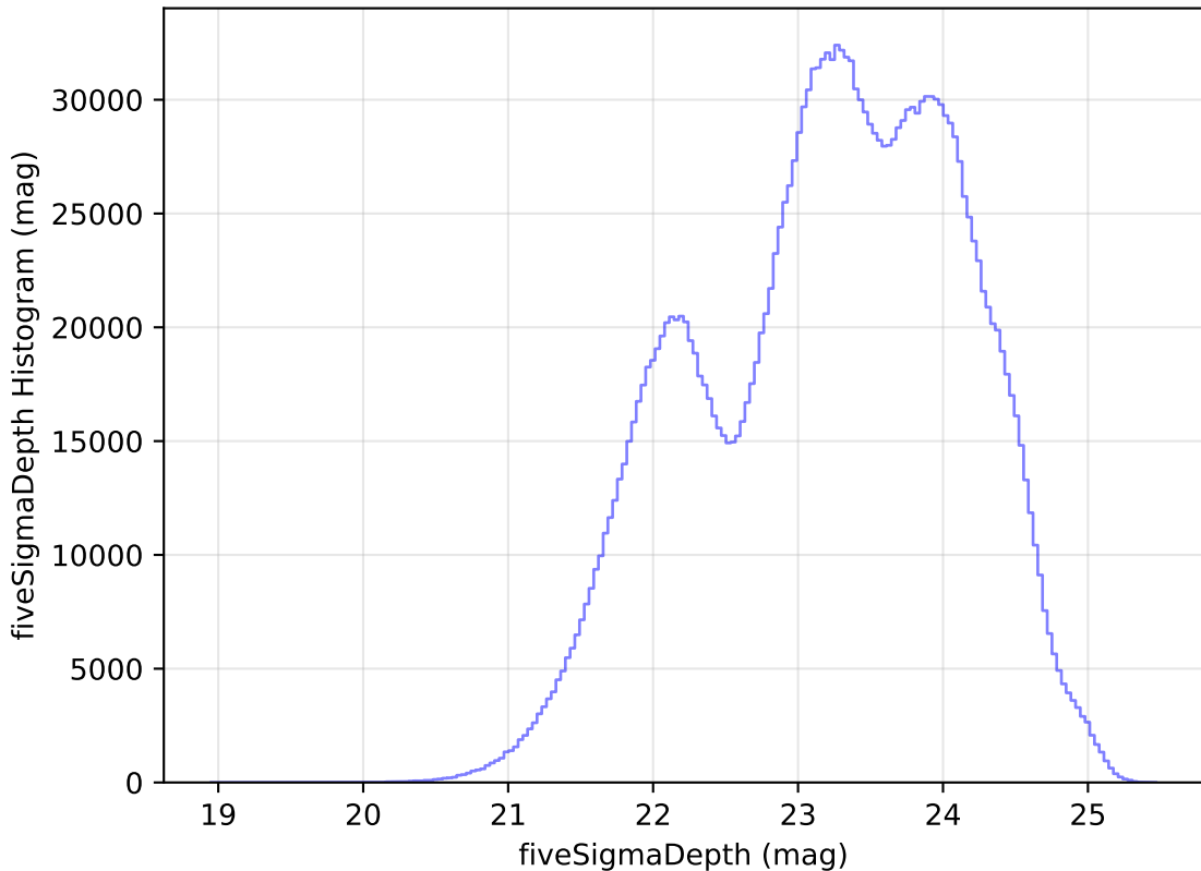
weather_cloudso20v3.4_10yrs WFD all bands: fiveSigmaDepth Histogram
