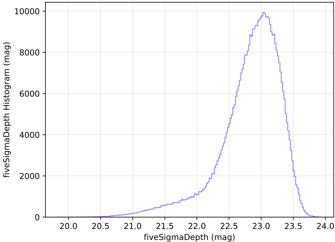
weather_cloudso20v3.4_10yrs All sky z band: fiveSigmaDepth Histogram
