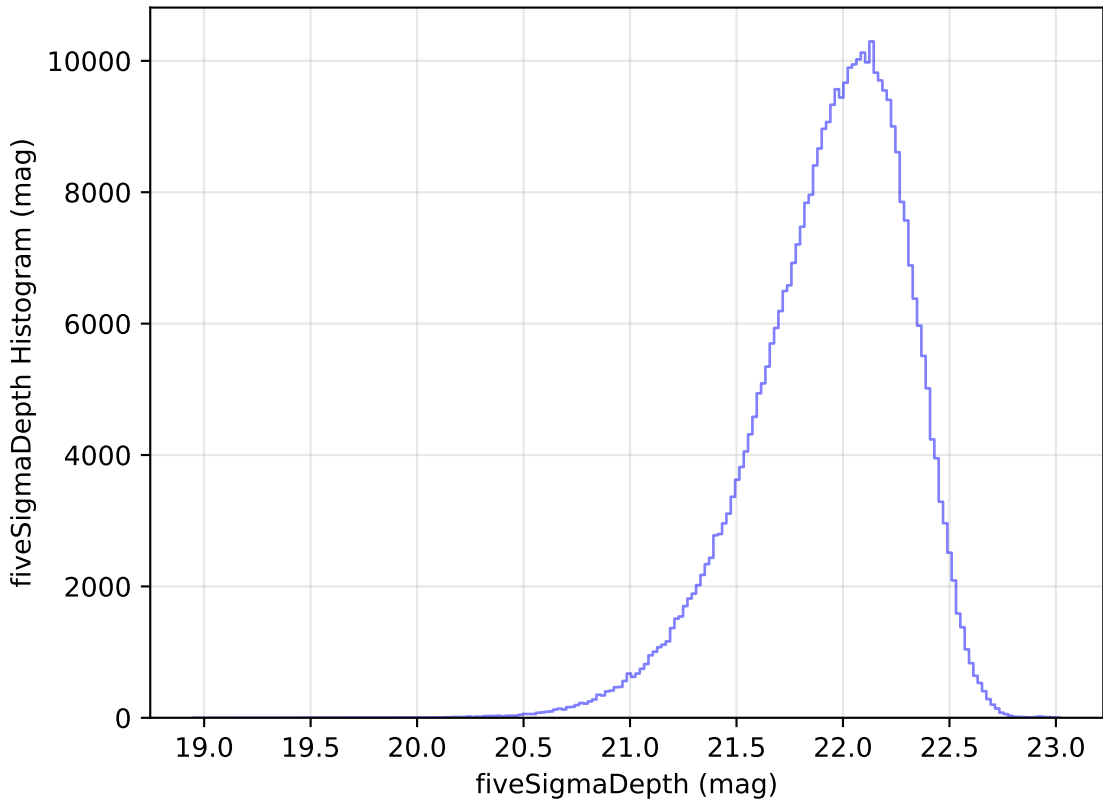
weather_cloudso20v3.4_10yrs All sky y band: fiveSigmaDepth Histogram
