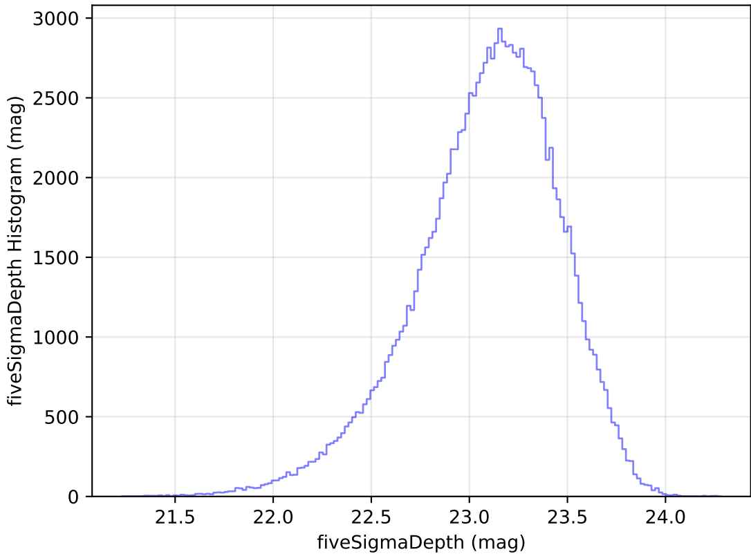
weather_cloudso20v3.4_10yrs All sky u band: fiveSigmaDepth Histogram
