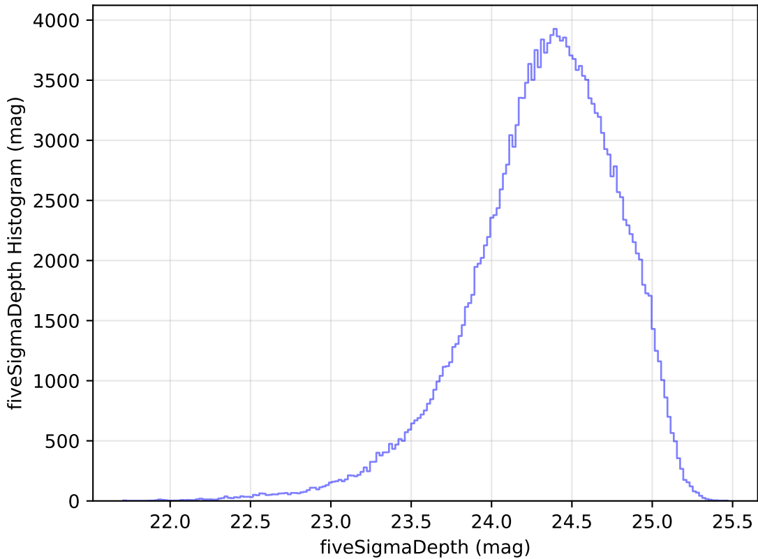
weather_cloudso20v3.4_10yrs All sky g band: fiveSigmaDepth Histogram
