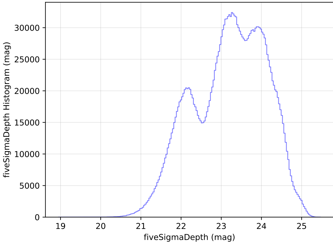
weather_cloudso20v3.4_10yrs All sky all bands: fiveSigmaDepth Histogram
