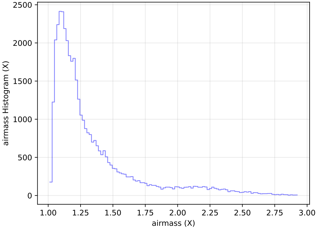
weather_cloudso20v3.4_10yrs Yr 1 z band: airmass Histogram
