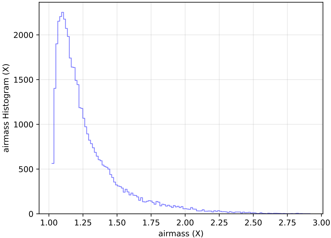
weather_cloudso20v3.4_10yrs Yr 1 y band: airmass Histogram
