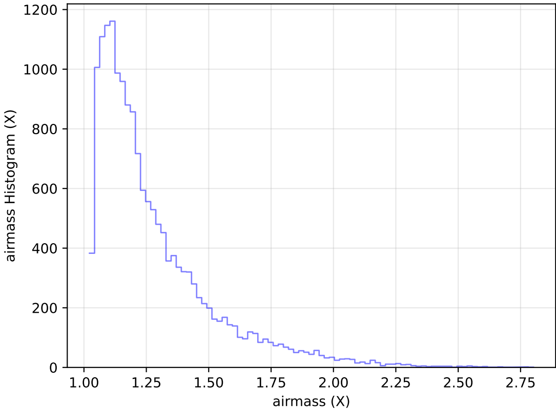
weather_cloudso20v3.4_10yrs Yr 1 u band: airmass Histogram
