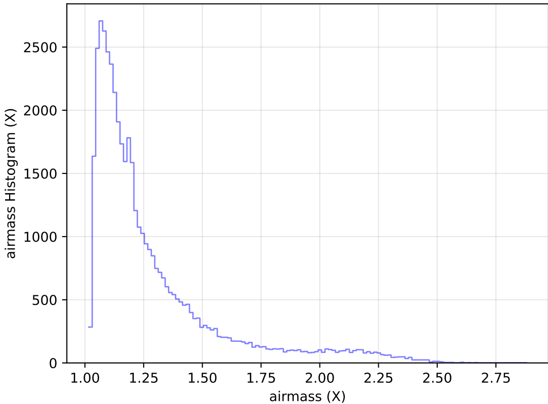
weather_cloudso20v3.4_10yrs Yr 1 r band: airmass Histogram
