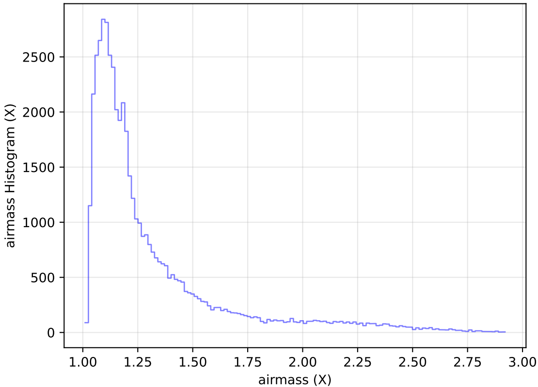
weather_cloudso20v3.4_10yrs Yr 1 i band: airmass Histogram
