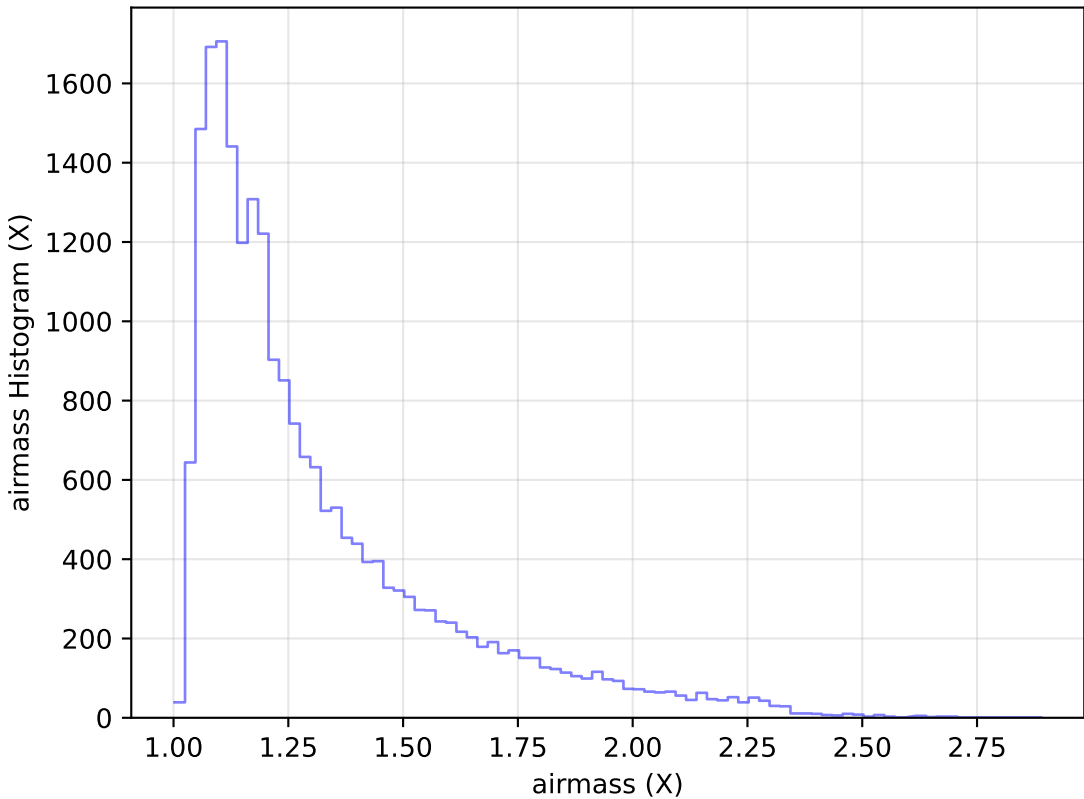
weather_cloudso20v3.4_10yrs Yr 1 g band: airmass Histogram
