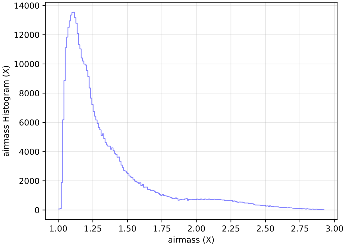
weather_cloudso20v3.4_10yrs WFD z band: airmass Histogram
