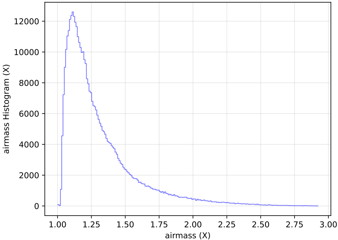
weather_cloudso20v3.4_10yrs WFD y band: airmass Histogram
