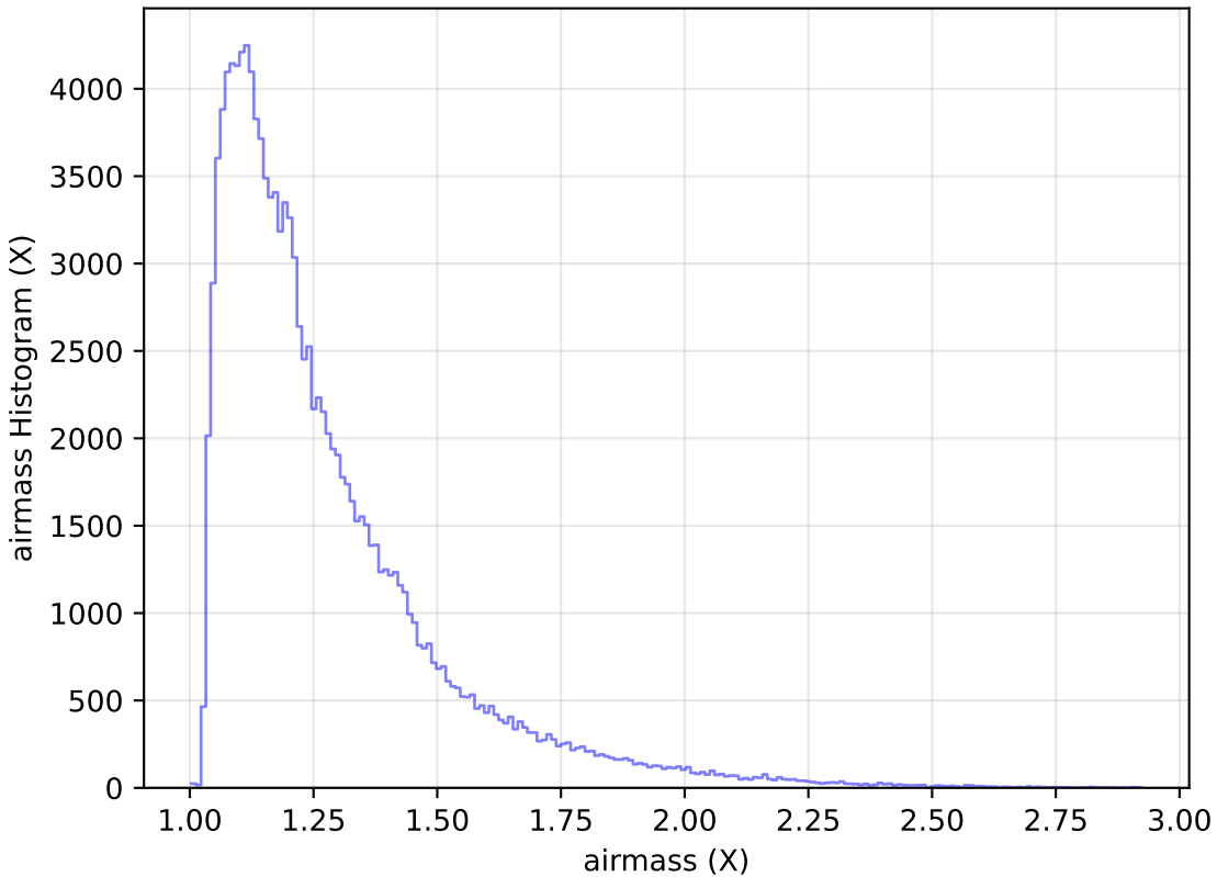
weather_cloudso20v3.4_10yrs WFD u band: airmass Histogram
