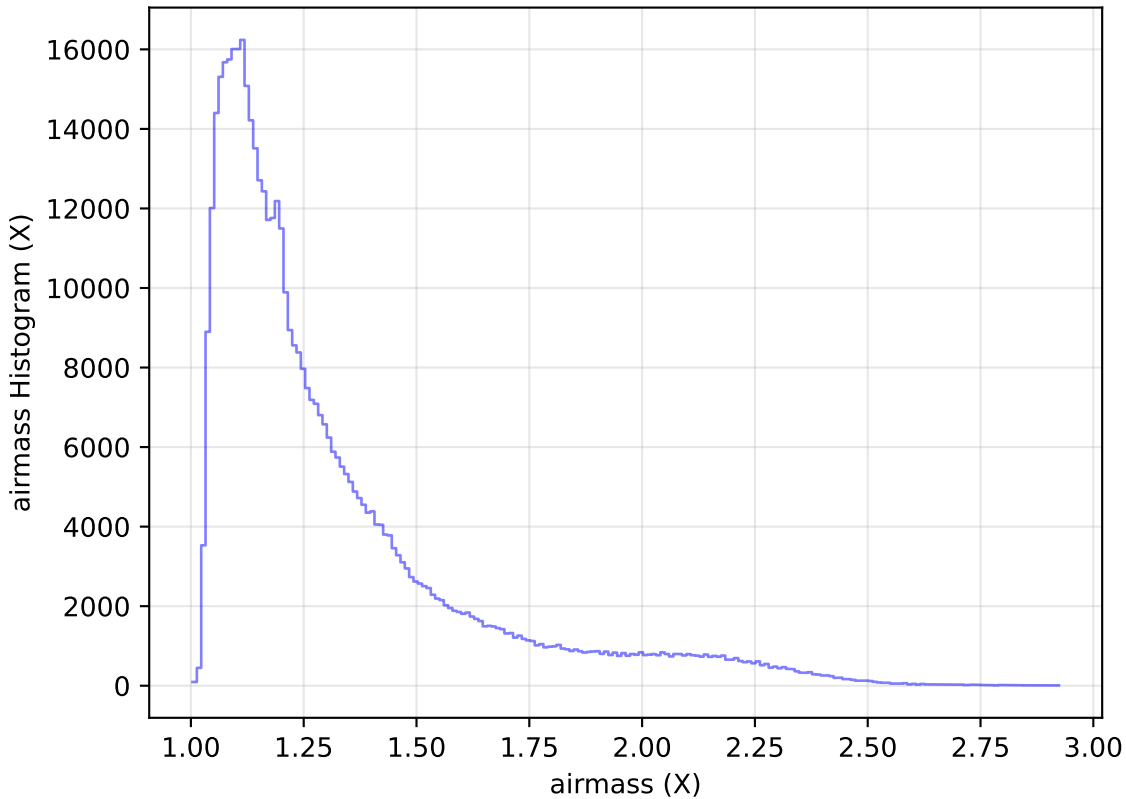
weather_cloudso20v3.4_10yrs WFD r band: airmass Histogram
