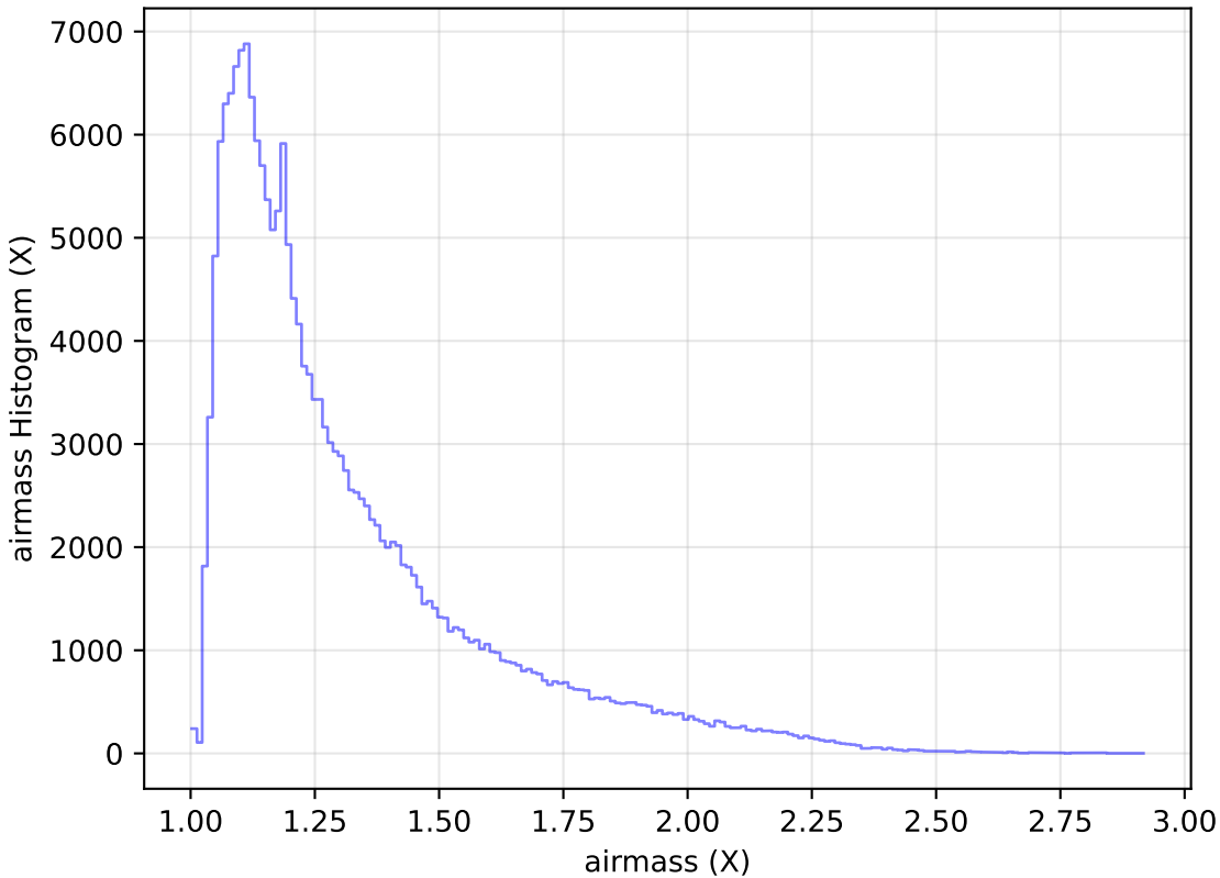
weather_cloudso20v3.4_10yrs WFD g band: airmass Histogram
