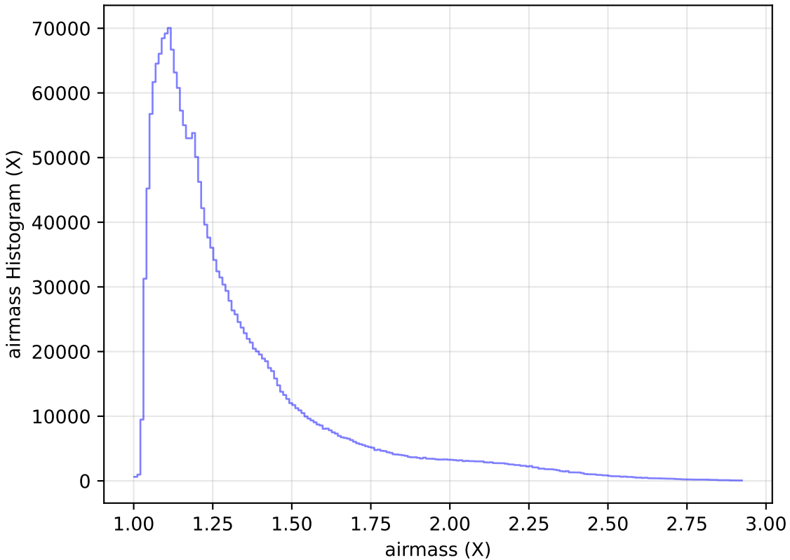
weather_cloudso20v3.4_10yrs WFD all bands: airmass Histogram
