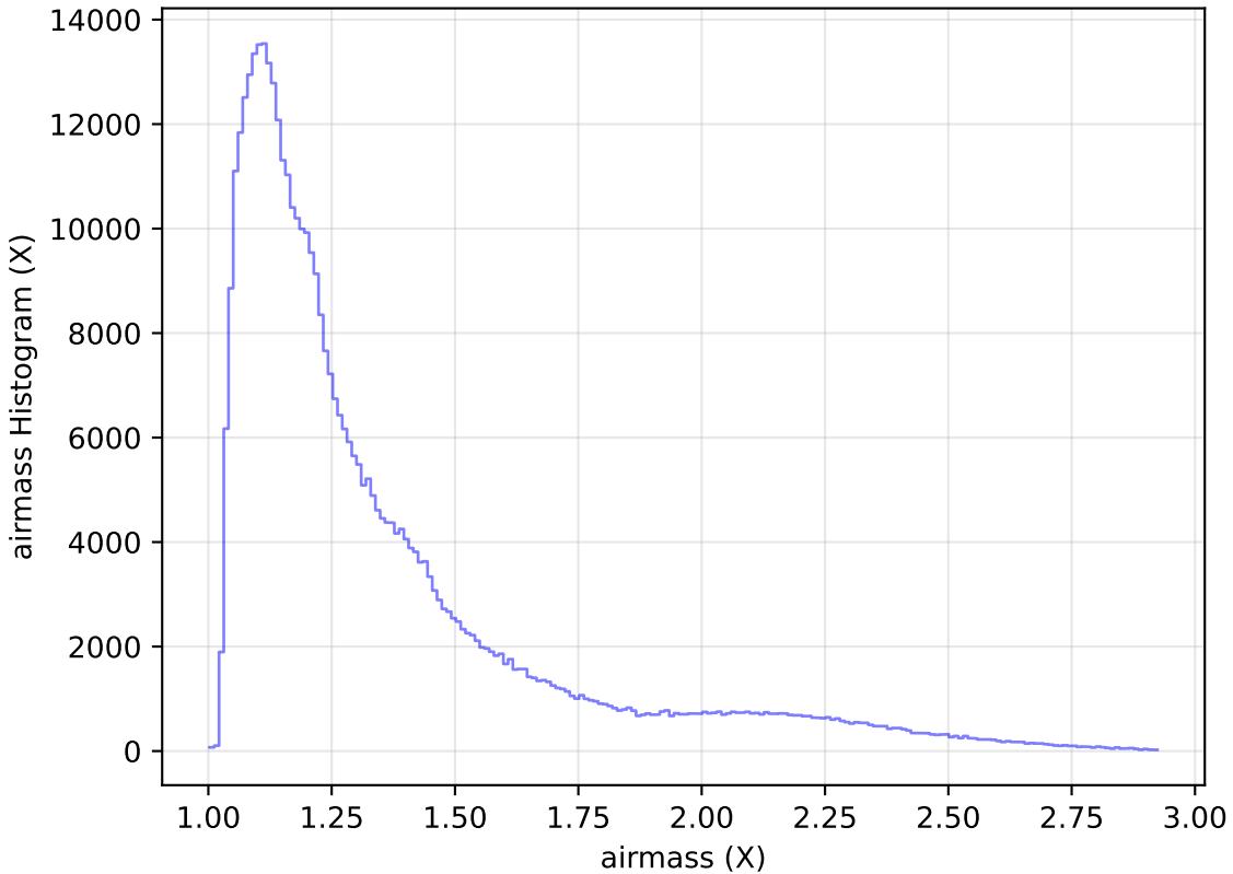
weather_cloudso20v3.4_10yrs All sky z band: airmass Histogram
