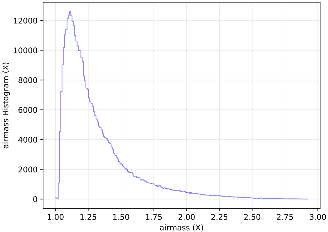
weather_cloudso20v3.4_10yrs All sky y band: airmass Histogram
