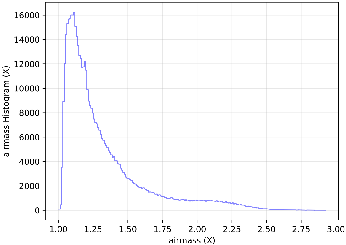
weather_cloudso20v3.4_10yrs All sky r band: airmass Histogram
