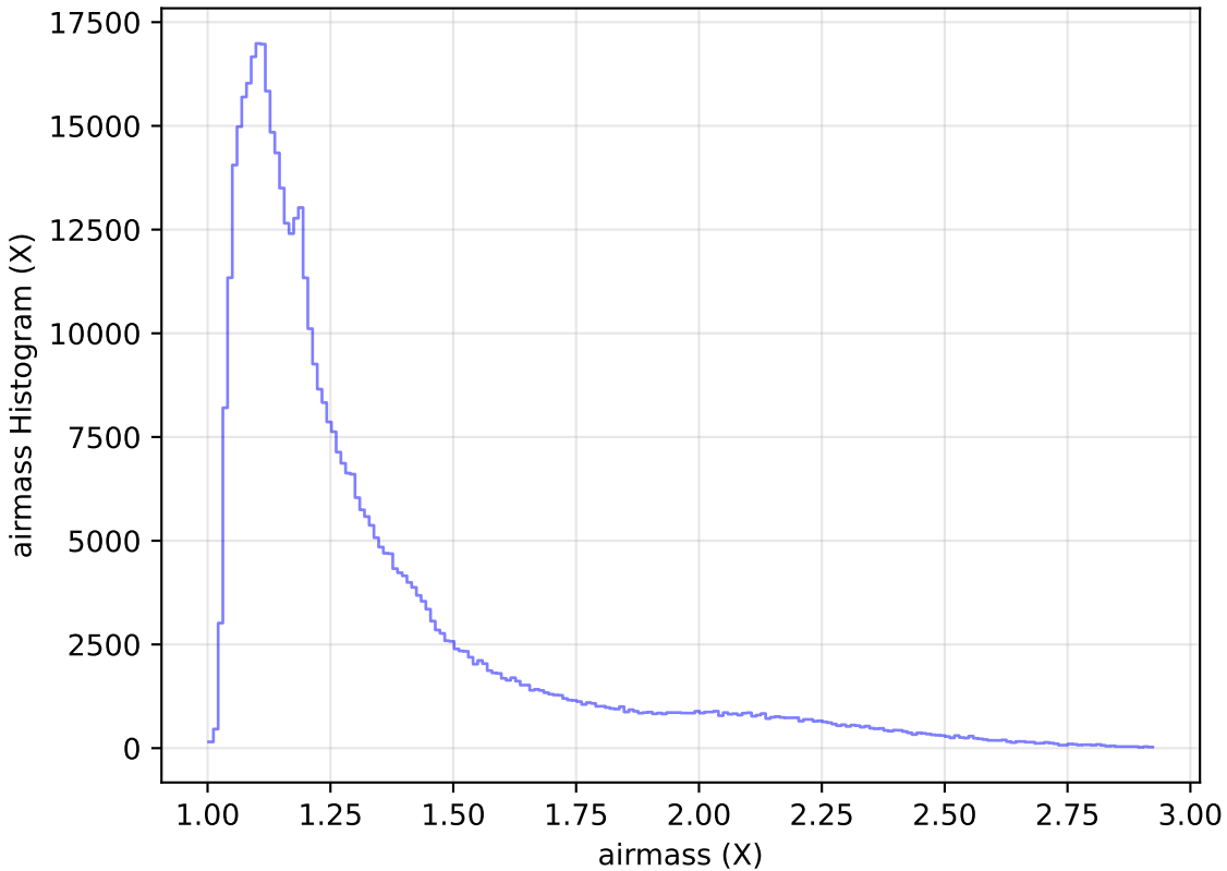
weather_cloudso20v3.4_10yrs All sky i band: airmass Histogram
