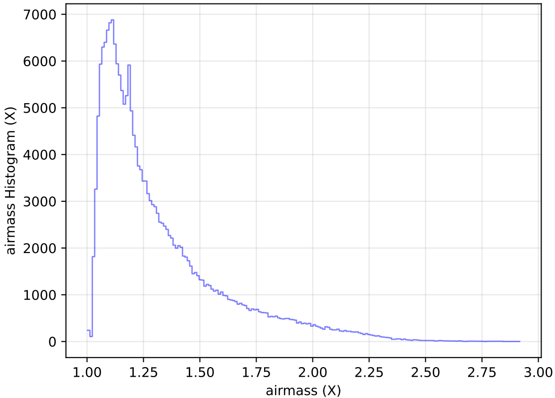
weather_cloudso20v3.4_10yrs All sky g band: airmass Histogram
