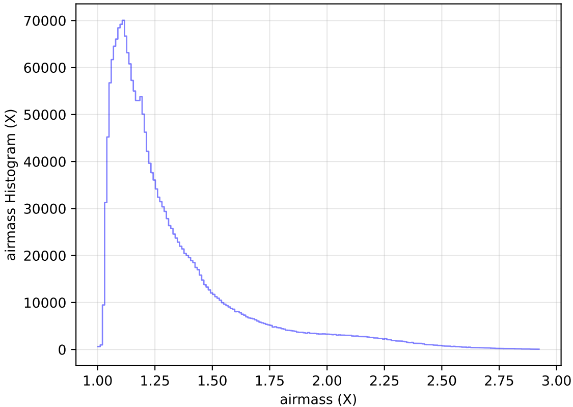
weather_cloudso20v3.4_10yrs All sky all bands: airmass Histogram
