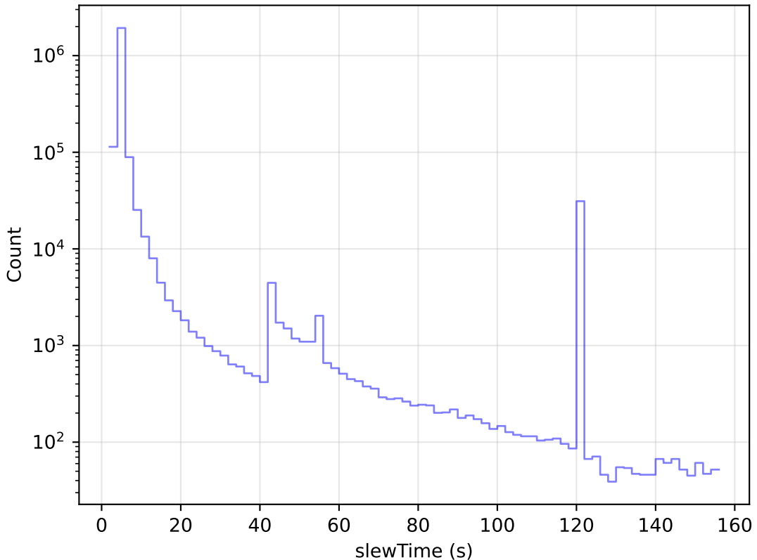
weather_cloudso20v3.4_10yrs All visits: Slew Time Histogram
