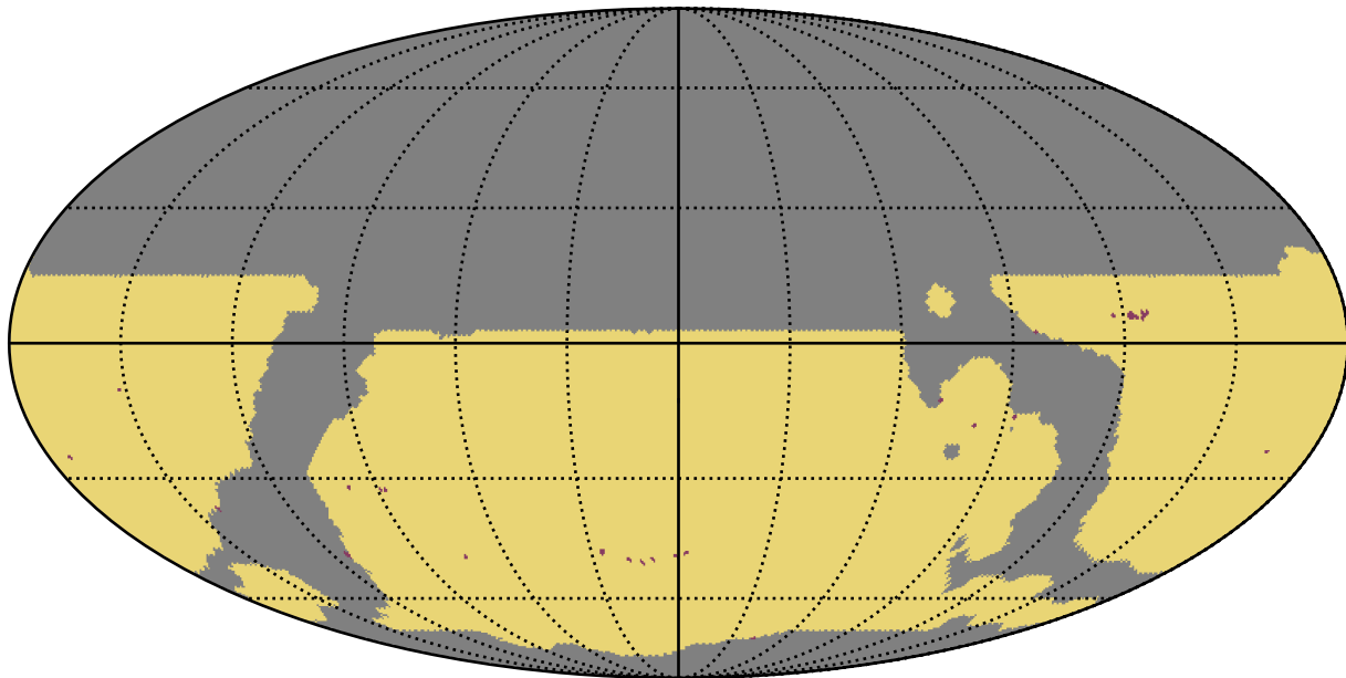
weather_cloudso20v3.4_10yrs WFD: RapidRevisits
