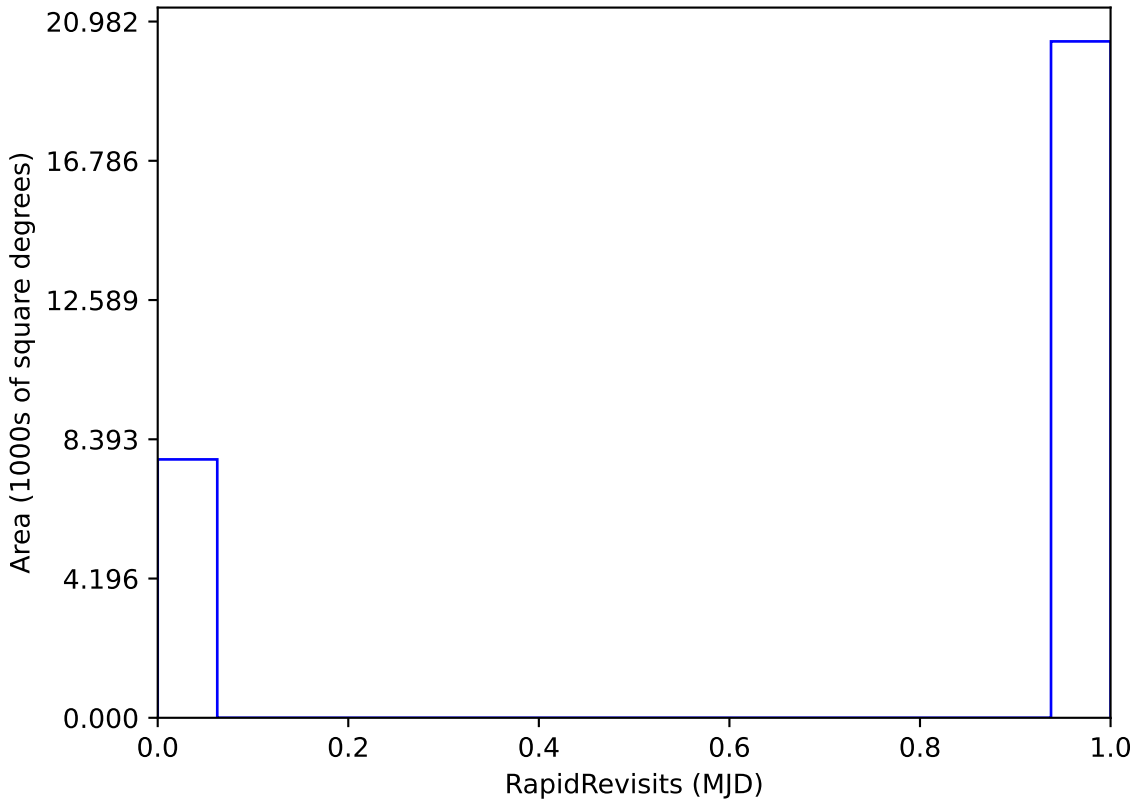
weather_cloudso20v3.4_10yrs All sky: RapidRevisits
