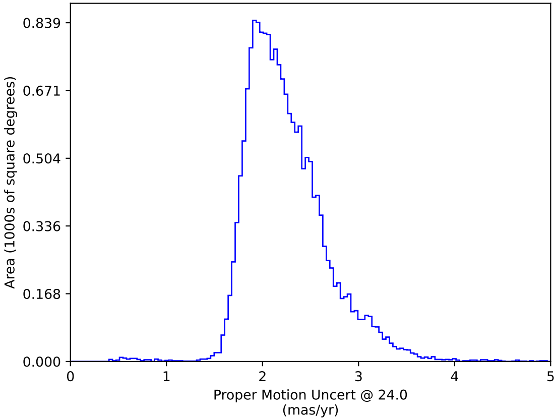
weather_cloudso20v3.4_10yrs WFD: Proper Motion Uncert @ 24.0
