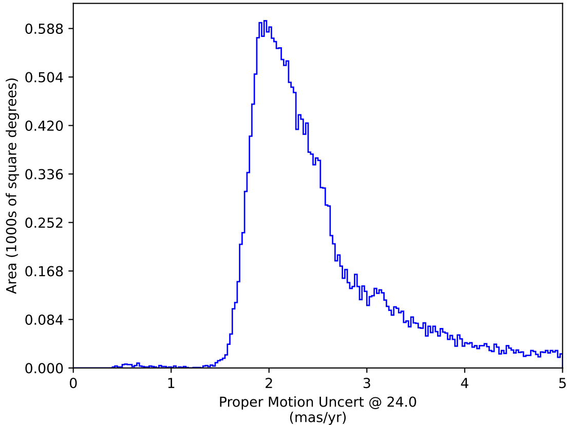
weather_cloudso20v3.4_10yrs All sky: Proper Motion Uncert @ 24.0
