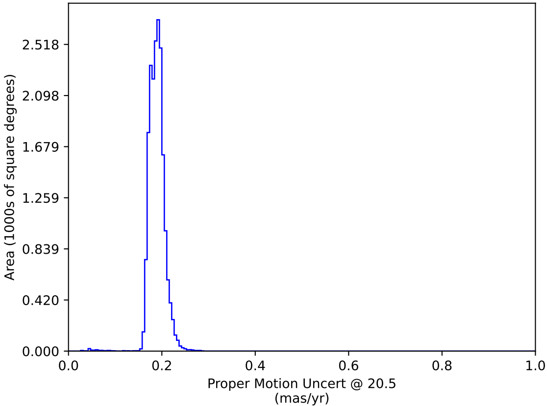
weather_cloudso20v3.4_10yrs WFD: Proper Motion Uncert @ 20.5
