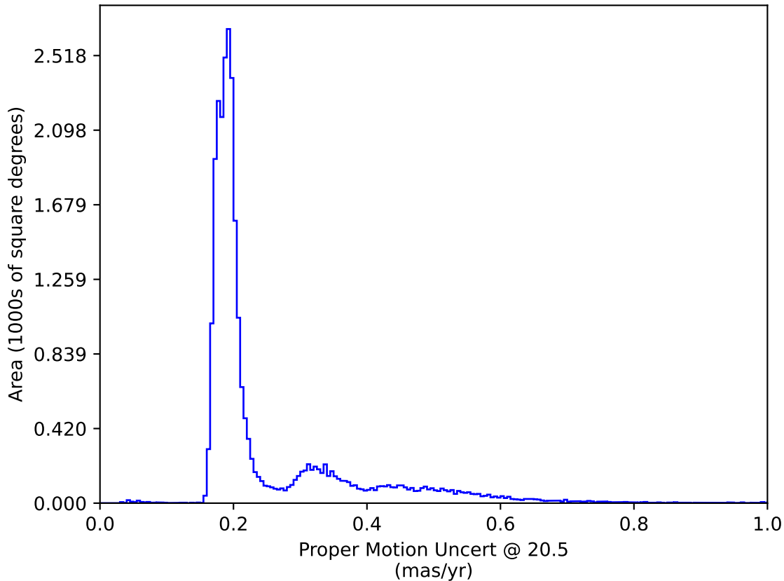
weather_cloudso20v3.4_10yrs All sky: Proper Motion Uncert @ 20.5
