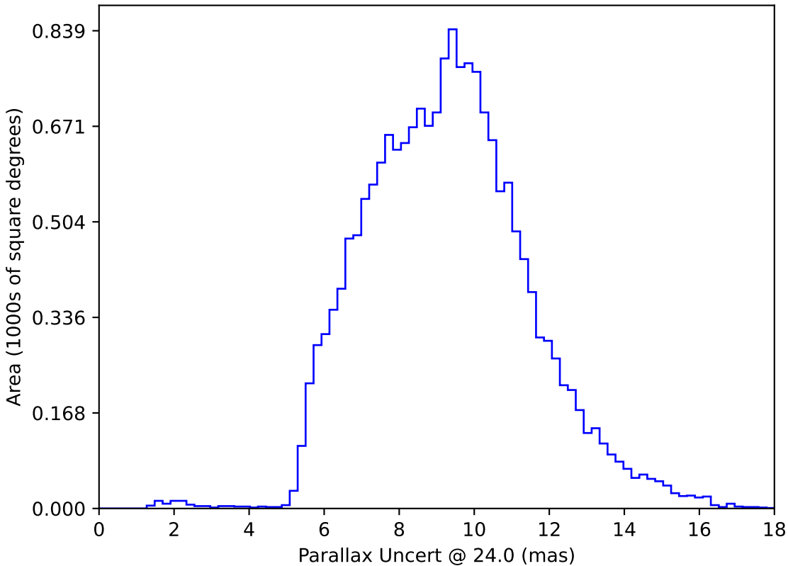
weather_cloudso20v3.4_10yrs WFD: Parallax Uncert @ 24.0
