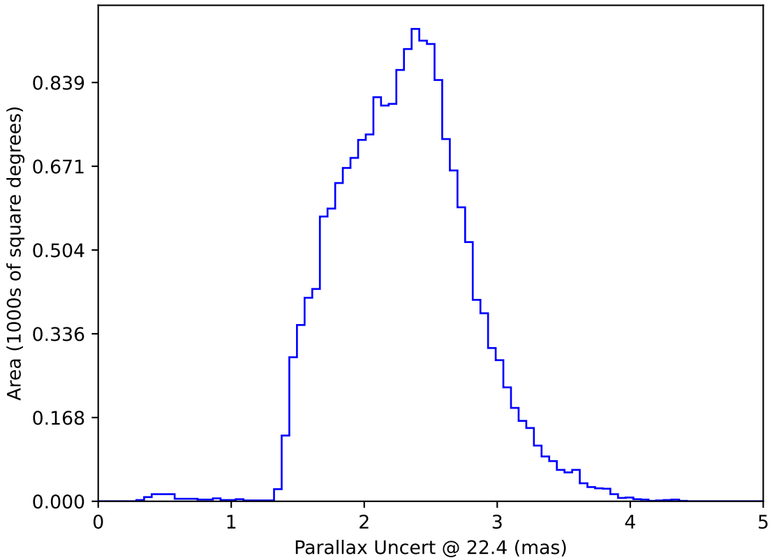
weather_cloudso20v3.4_10yrs WFD: Parallax Uncert @ 22.4
