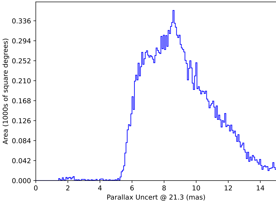
weather_cloudso20v3.4_10yrs All sky y band only: Parallax Uncert @ 21.3
