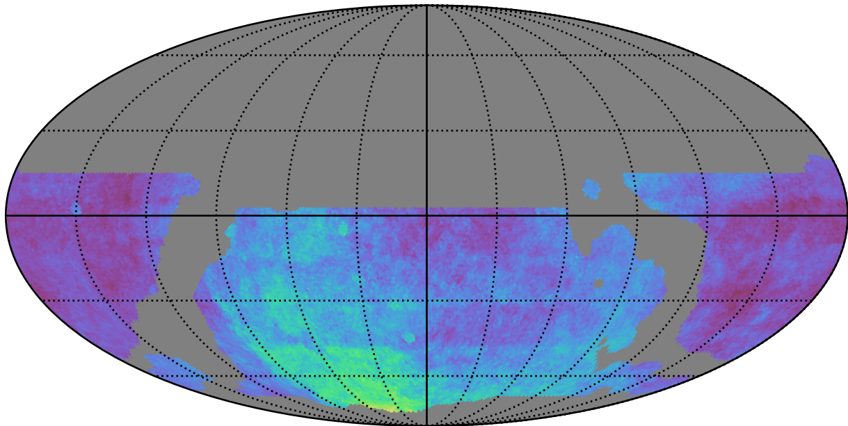
weather_cloudso20v3.4_10yrs WFD: Parallax Coverage @ 24.0
