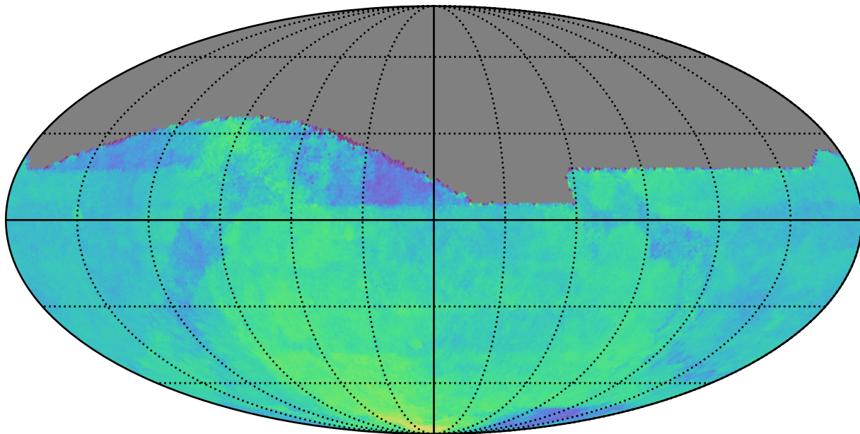
weather_cloudso20v3.4_10yrs All sky: Parallax Coverage @ 24.0
