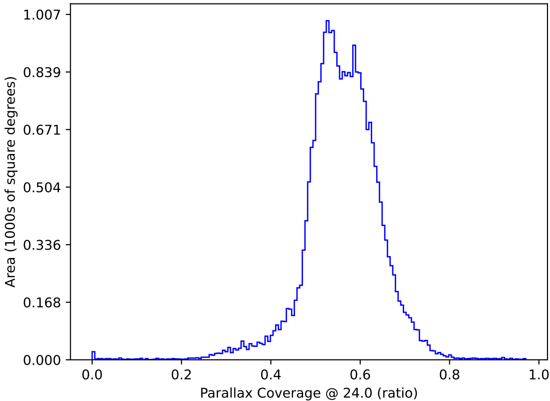
weather_cloudso20v3.4_10yrs All sky: Parallax Coverage @ 24.0
