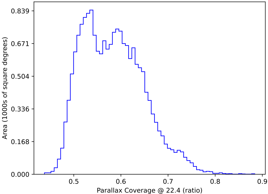
weather_cloudso20v3.4_10yrs WFD: Parallax Coverage @ 22.4
