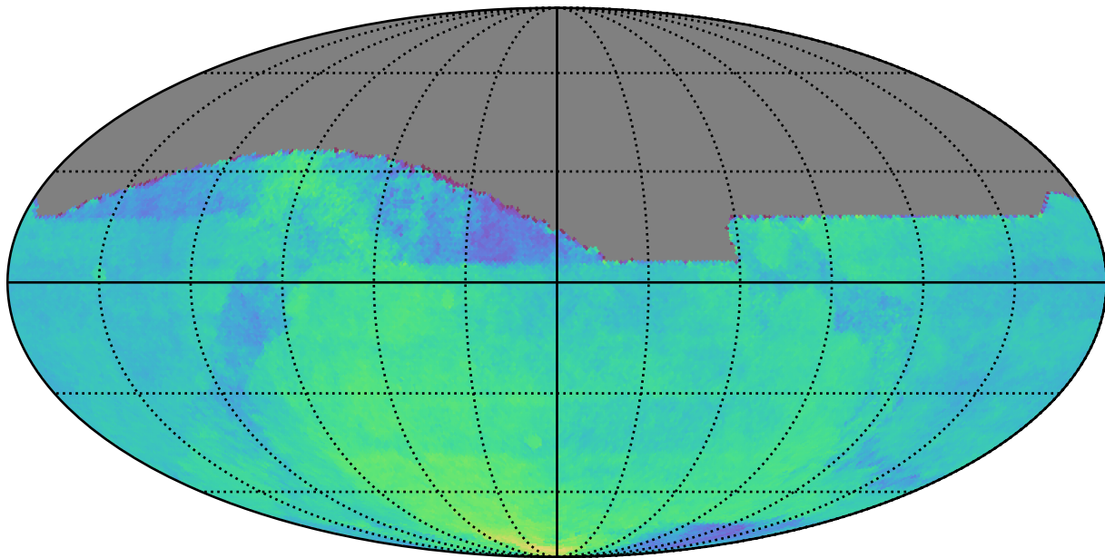
weather_cloudso20v3.4_10yrs All sky: Parallax Coverage @ 22.4
