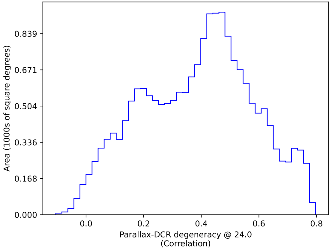
weather_cloudso20v3.4_10yrs WFD: Parallax-DCR degeneracy @ 24.0
