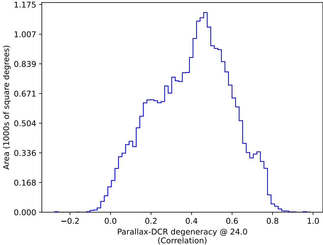
weather_cloudso20v3.4_10yrs All sky: Parallax-DCR degeneracy @ 24.0
