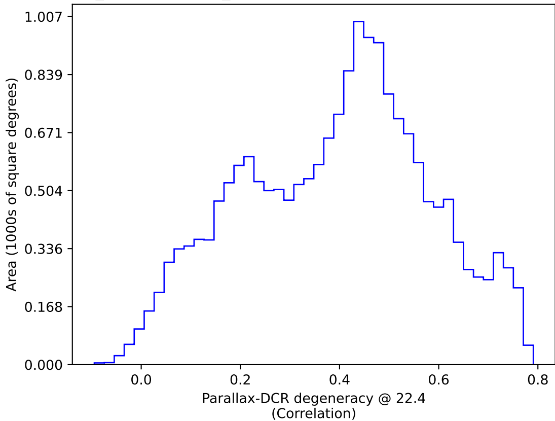
weather_cloudso20v3.4_10yrs WFD: Parallax-DCR degeneracy @ 22.4
