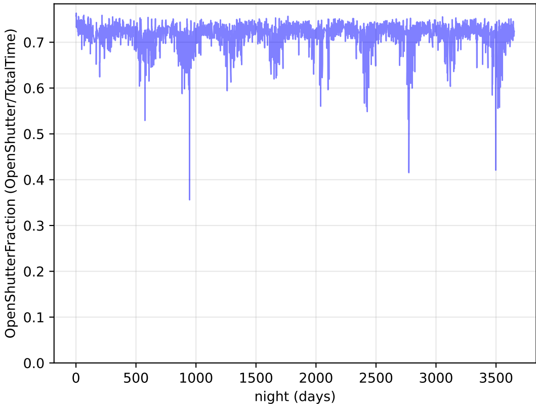
weather_cloudso20v3.4_10yrs Per night: OpenShutterFraction
