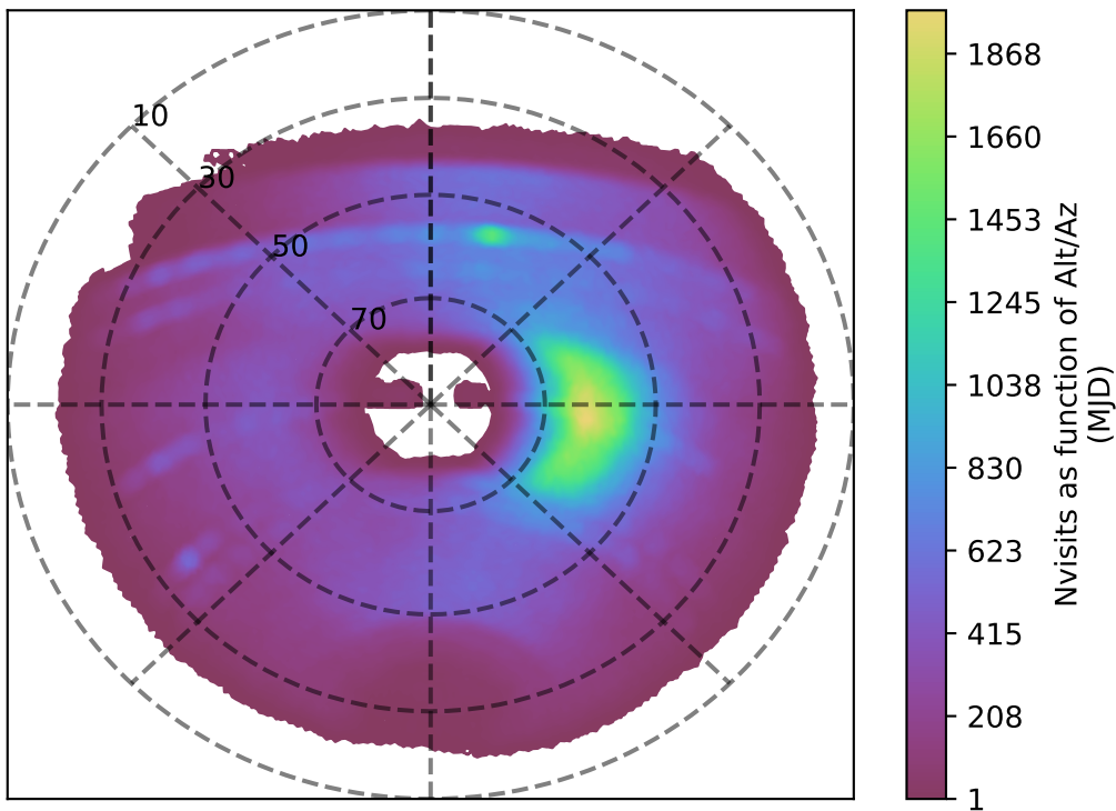
weather_cloudso20v3.4_10yrs y band: Nvisits as function of Alt/Az
